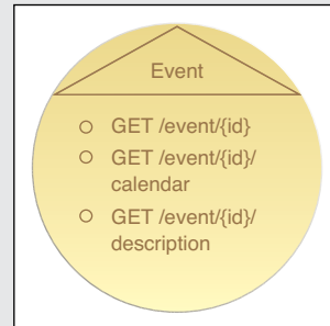
Figure 9.6 The Event service contract.
