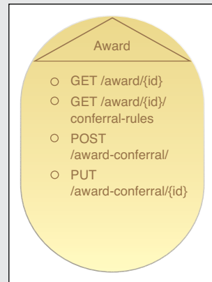
Figure 9.7 The Award service contract.
